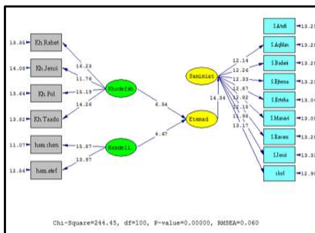
Figure 1 Diagram of tested structural equations model
