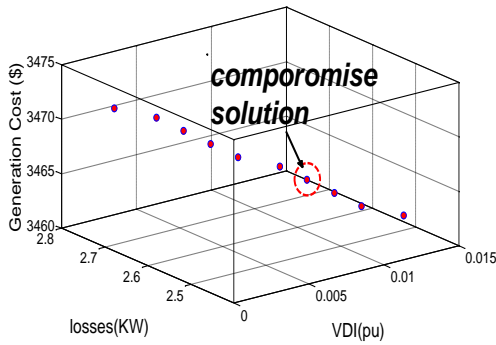
Fig. 1. Description of Pareto front in \varepsilon -constraint method.
